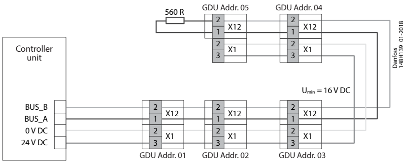
Figure: How to make proper connections between the controller and each GDU
