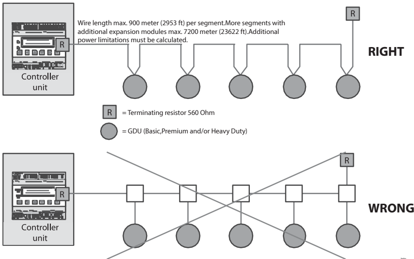
Figure: How to make proper connections between the controller and each GDU
