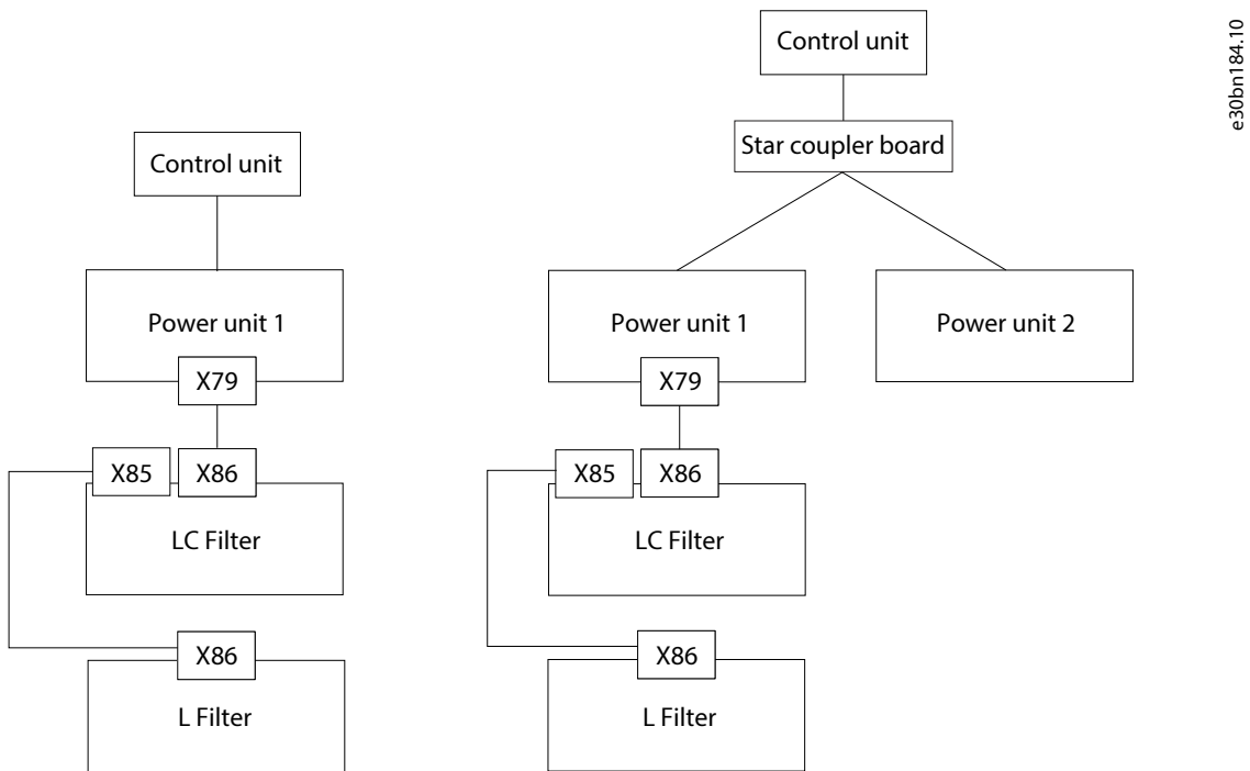
Figure 19: AuxBus Topology
