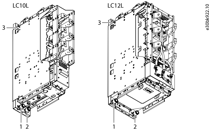
Figure 9: Location of the Cooling Circuit Connectors
