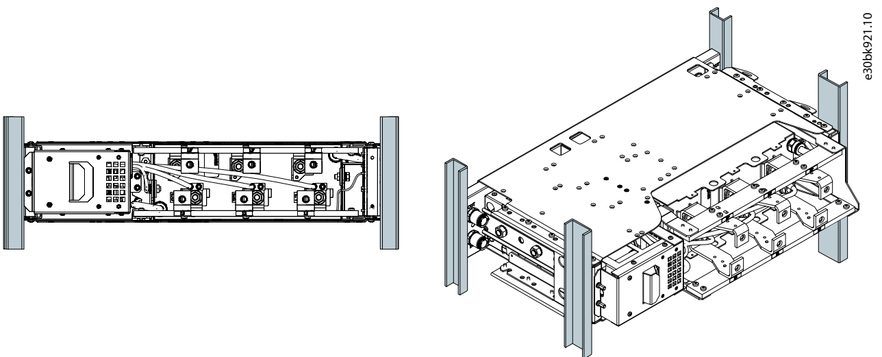
Figure 4: Example of Mounting the LC Filter Horizontally
