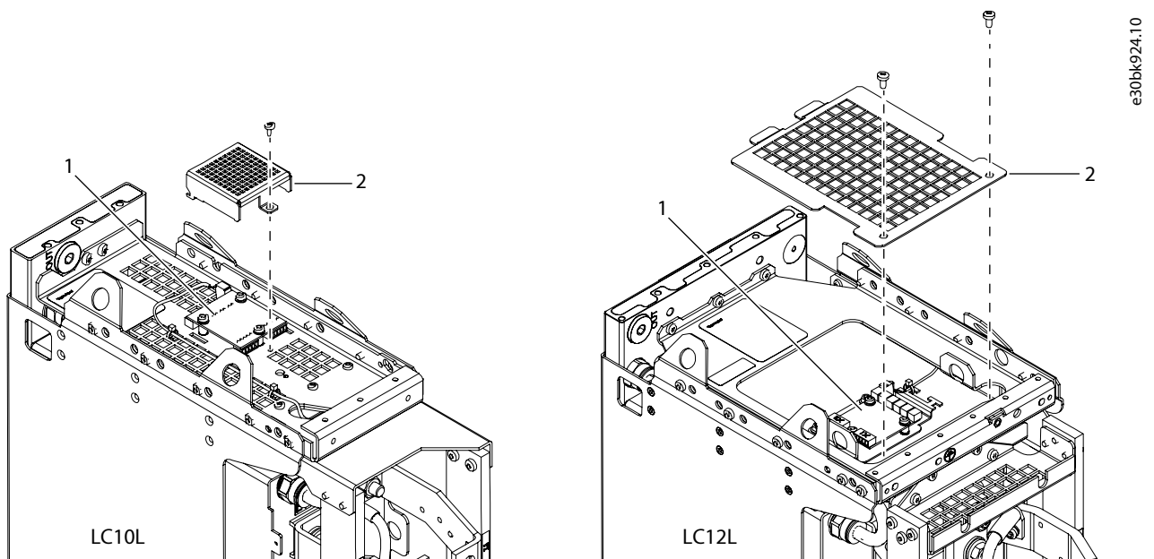
Figure 17: Accessing the AuxBus Temperature Measurement Board
