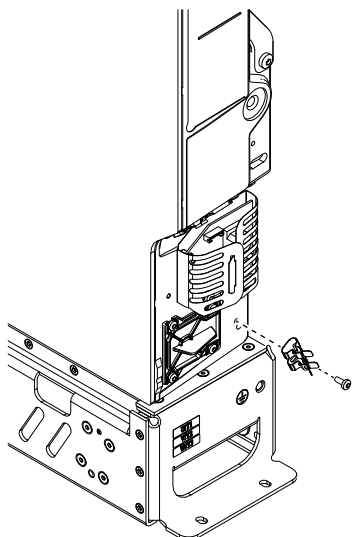
Figure 16: Mounting the Relief Plate
