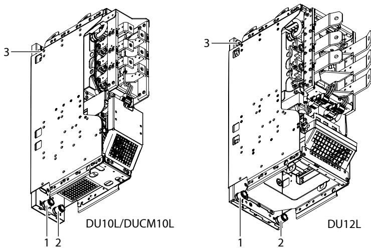
Figure 10: Location of the Cooling Circuit Connectors
