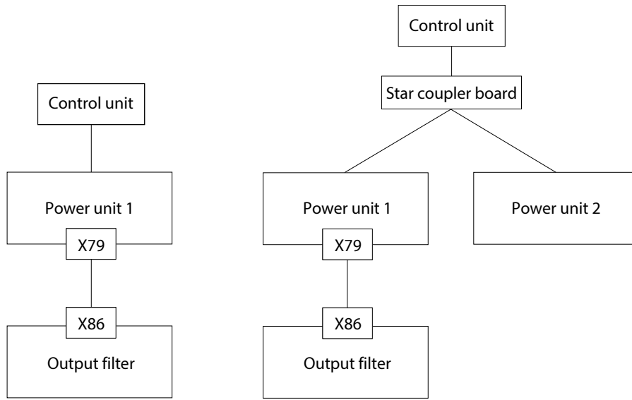
Figure 20: AuxBus Topology
