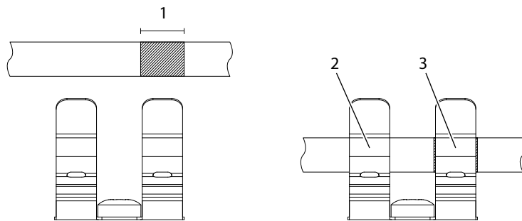
Figure 21: Using the Cable Clamps
