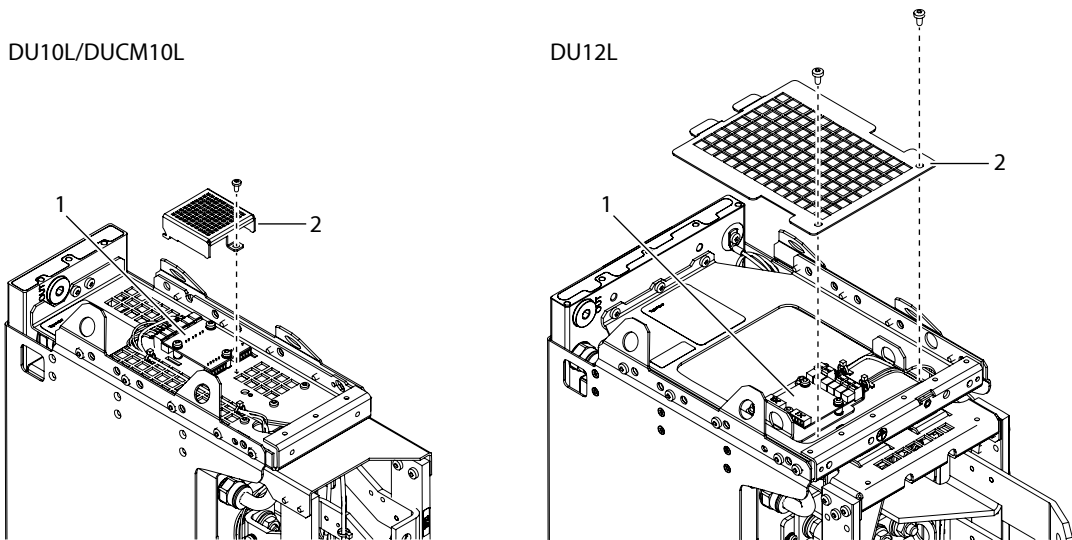
Figure 18: Accessing the AuxBus Temperature Measurement Board
