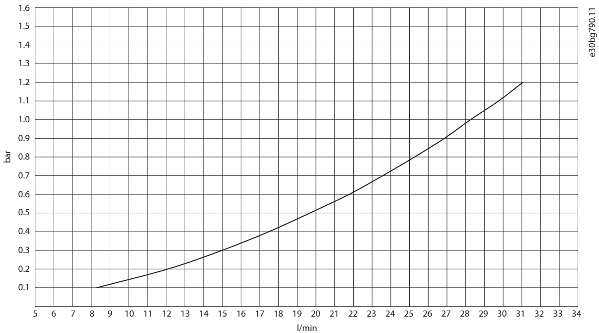
Figure 8: Pressure Drop with Water, dU/dt Filter OF7U1/OF7U2, DU10L/DUCM10L
