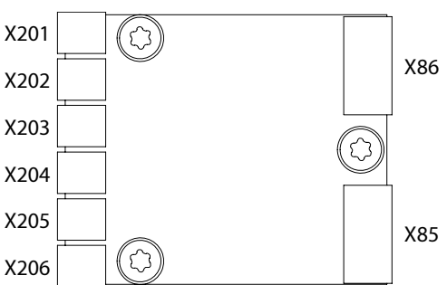
Figure 19: Terminals on the AuxBus Temperature Measurement Board
