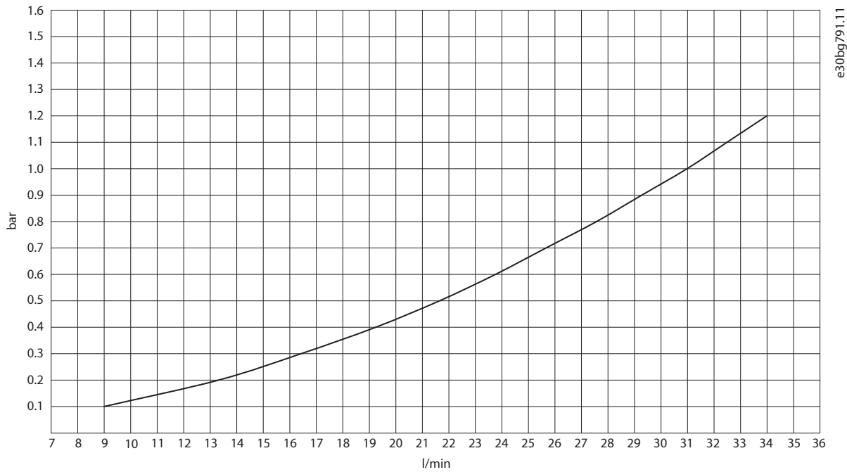
Figure 9: Pressure Drop with Water, dU/dt Filter OF7U1/OF7U2, DU12L
