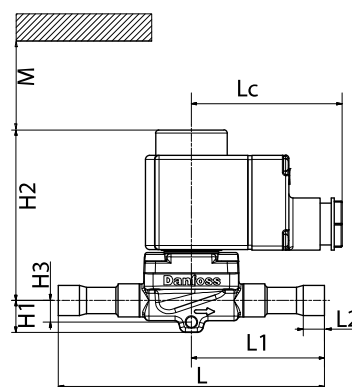
Figure: EVR and Terminal box coil
