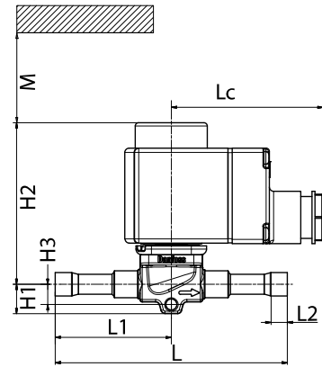
Figure: EVR and Terminal box coil
