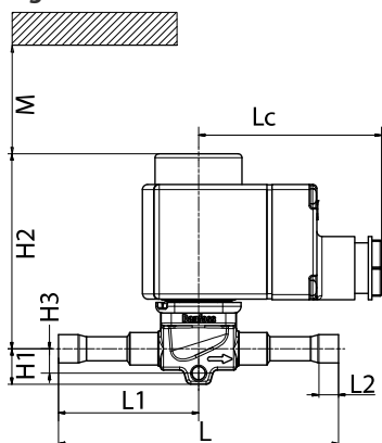
Figure: EVRC and Terminal box coil
