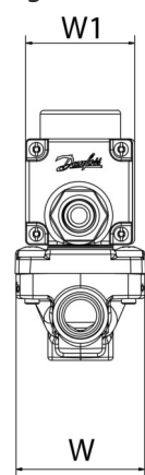
Figure: End view
