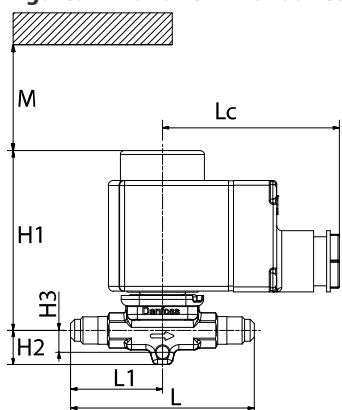
Figure: EVR and Terminal box coil
