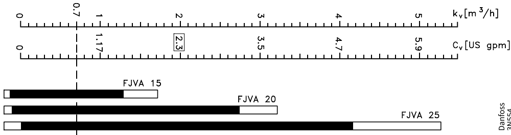
Figure: Nomogram showing the valve k_v range
