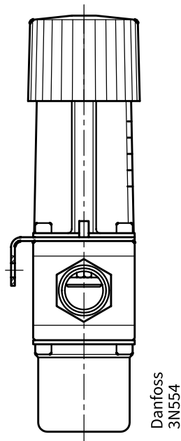
Figure: FJVA installation
