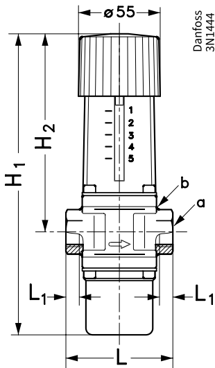
Figure: Dimensions and weights
