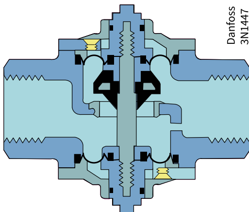
Figure: Valve body with by-pass
