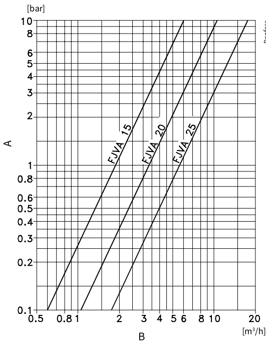
Figure: Valve flow quantity in fully open position, as a function of pressure drop \Delta p .
