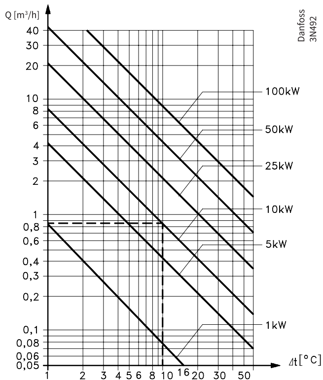
Figure: Heating or cooling with water
